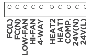
Terminal of PTAC Wall Thermostat (MODE B)
