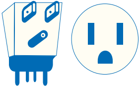
LCDI (NEMA 5-15P) 115V 15A
